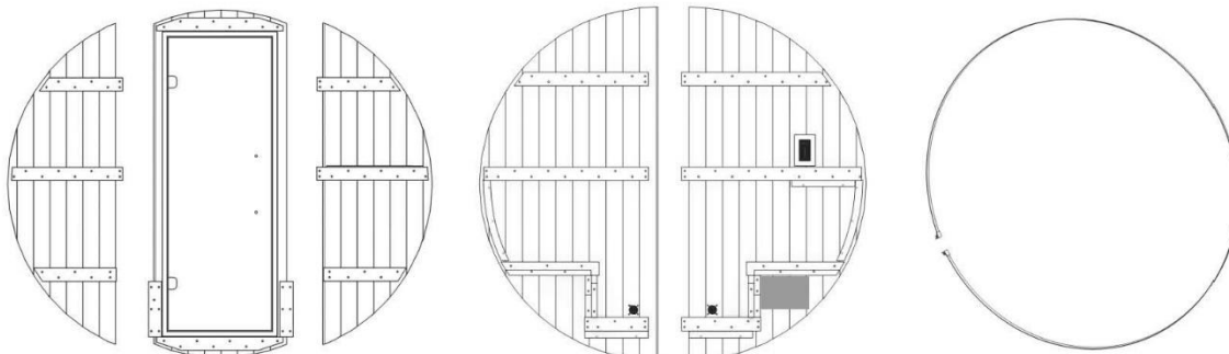
11 Front wall panel 12 Rear wall panel 13 Stainless steel band
