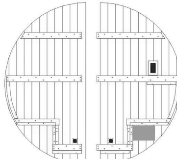
12 1794*905*30+20+20=2 (M4*40=6) Rear wall panel
